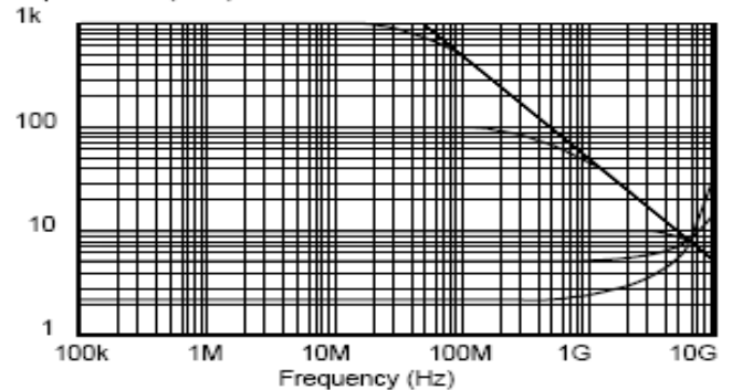
Impedance (ohm)
