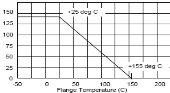
Rating Power(W)
