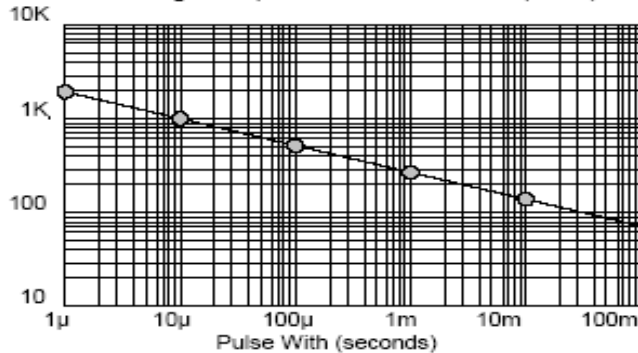
One time rectangular impulse. Pulse Peak Watt (Watts)
