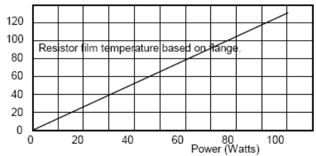
Temperature Rise Temperature Rise (C)
