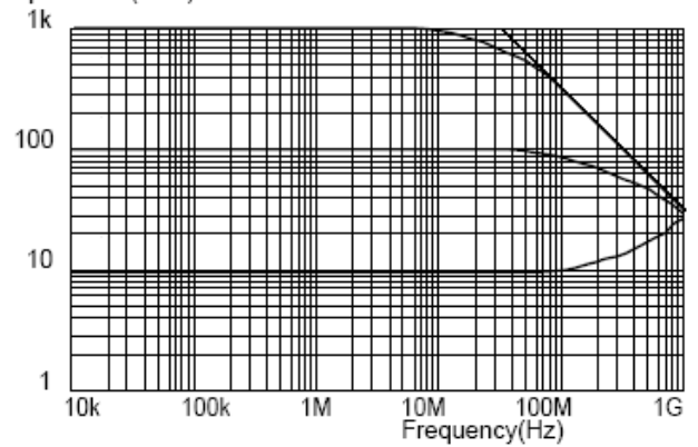
Frequency Characteristics Impedance (ohm)
