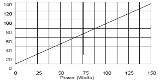
Resistor surface temperature rise based on flange (deg C)
