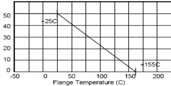
Rating Power (W)
