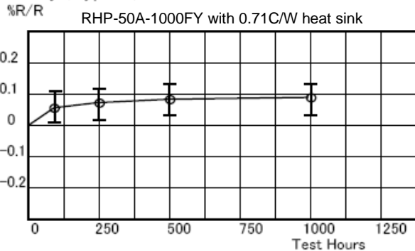
Humidity (Typical)
