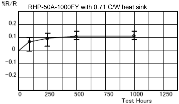
Load Life (Typical) %R/R Test Hours
