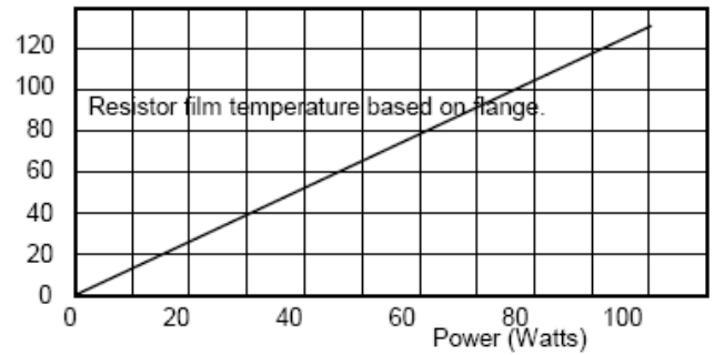
Temperature Rise Temperature Rise (°C) Power (Watts)
