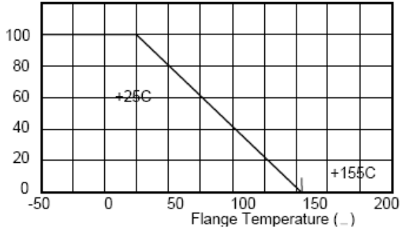
Derating Curve Rating Power(W) Flange Temperature (°C)
