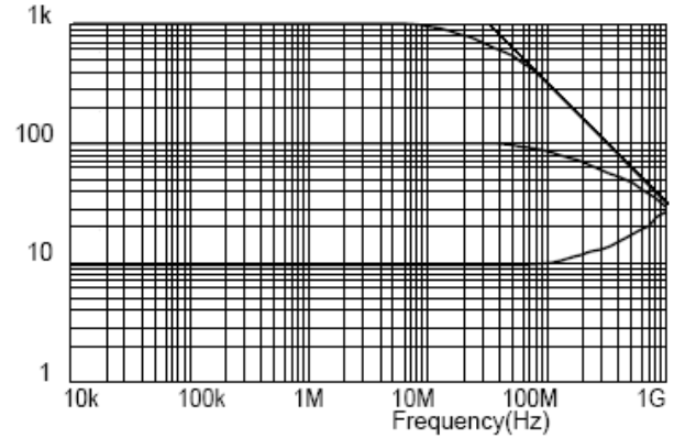
Frequency Characteristics Impedance (ohm) Frequency (Hz)
