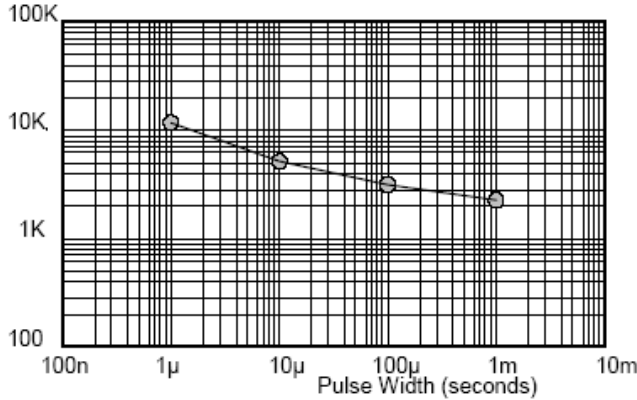
Pulse Energy Durability Pulse Peak Watt (Watts) Pulse Width (seconds)
