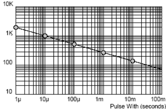
Pulse Energy Durability
