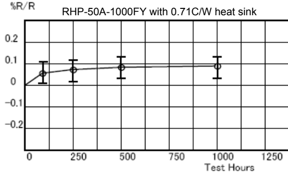
Humidity (Typical) %R/R Test Hours
