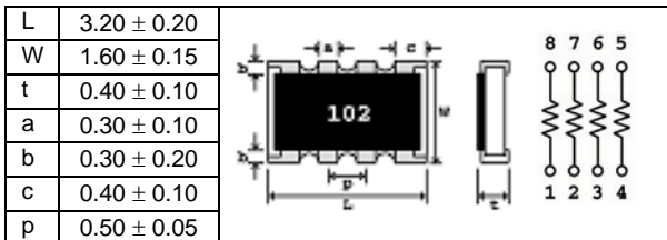
CRN16-4V Convex-Square
