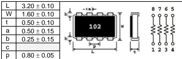
CRN16-4V Convex-Round
