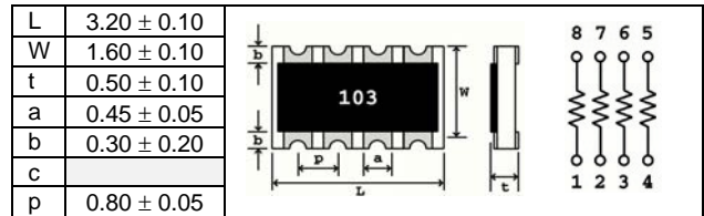
CRN16-4V Concave
