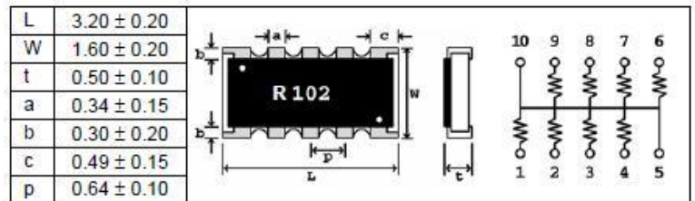
CRN16-8SU Convex-Square
