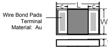
Top Side Termination, Bottom Isolated CRG, CJG type
